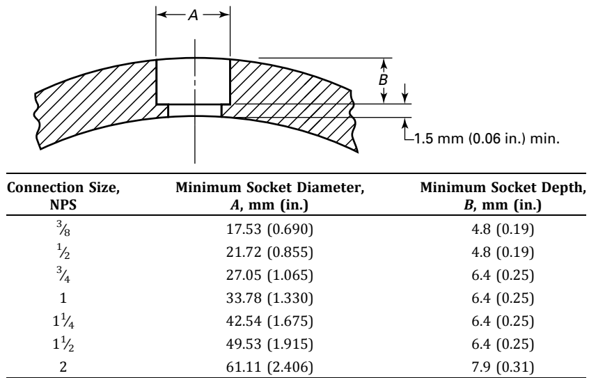
Figure 5 Socket Welding for Auxiliary Connections
