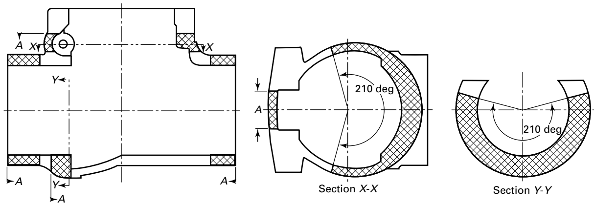
Figure 19 Swing Check
