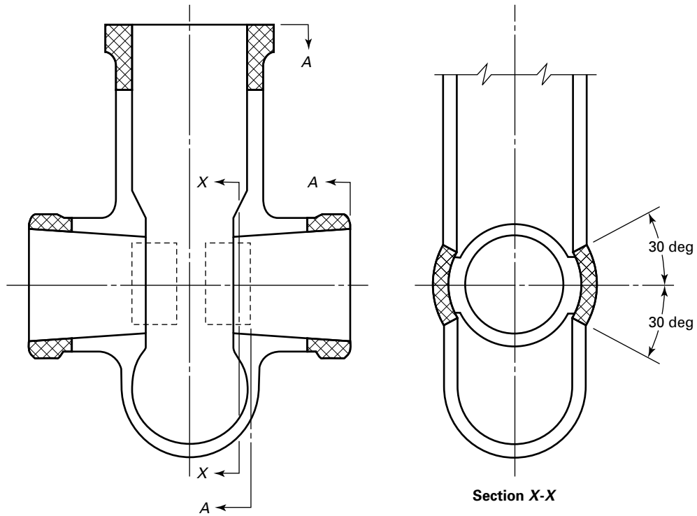
Figure 15 Conduit Gate Body (Pressure Seal Bonnet)
